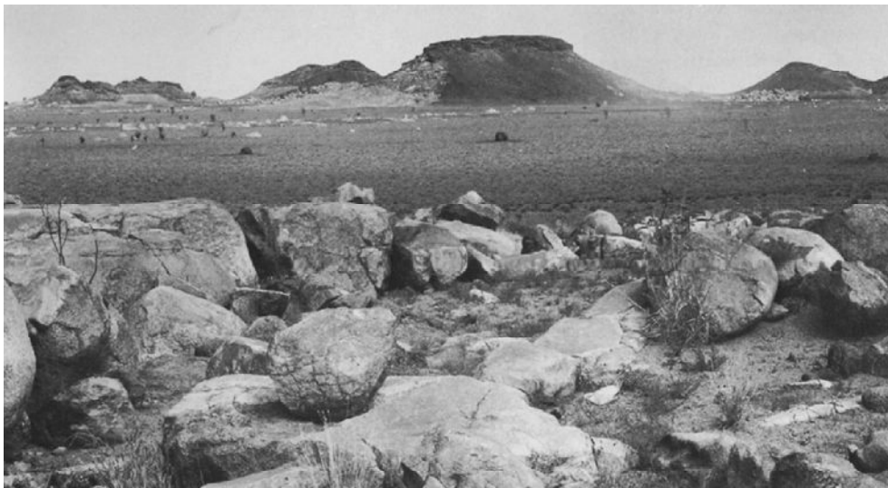
Fig. 4. Boulder-strewn granite hills in process of exposure from beneath flat-lying Cretaceous sediments east of Karratha, Western Australia.
